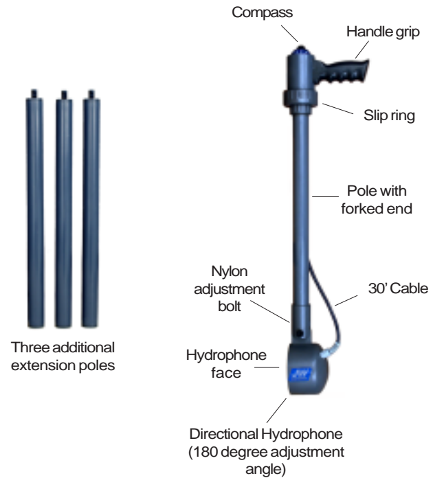
Boat Deployment Kit Option
