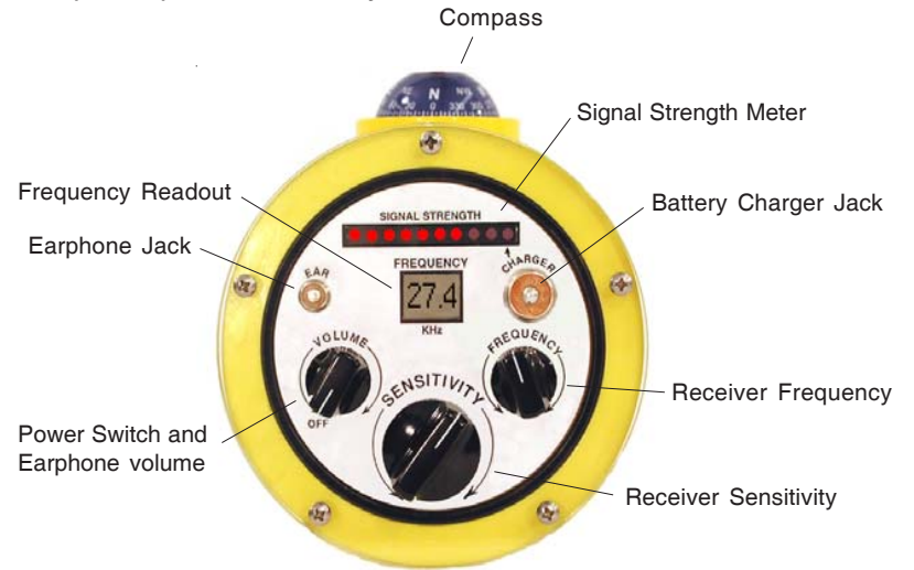
PR-1 FACEPLATE VIEW
