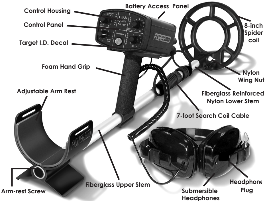
Figure 2. CZ-21 Quicksilver Detector.
