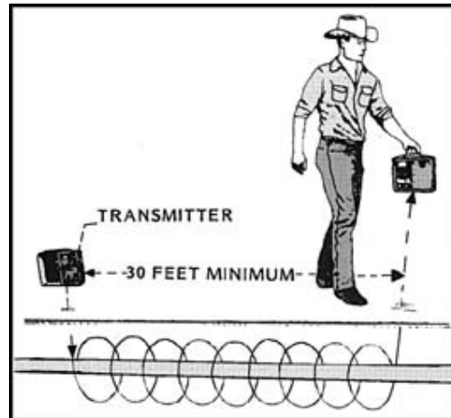
Figure 8. Inductive Trace
